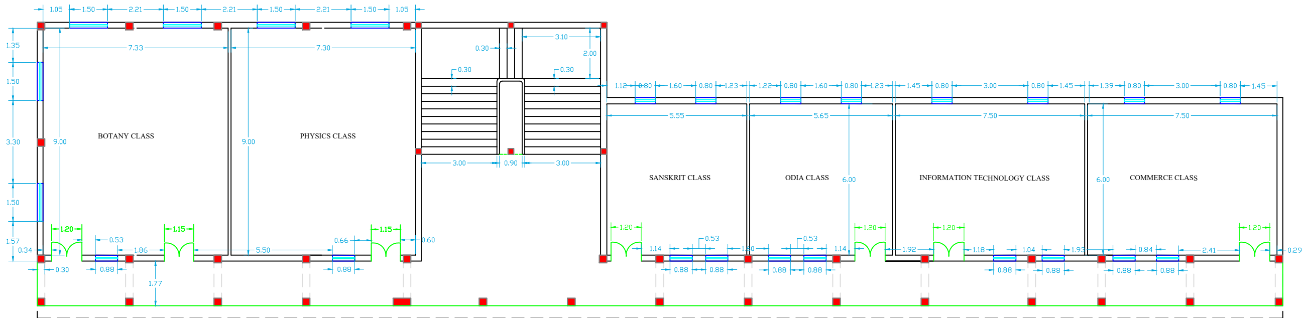
SCIENCE BLOCK - FIRST FLOOR
